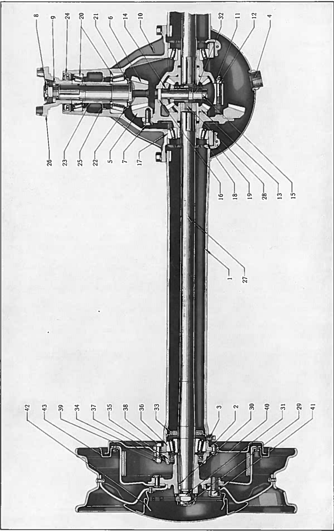
Figure 1301—Rear Axle Assembly
