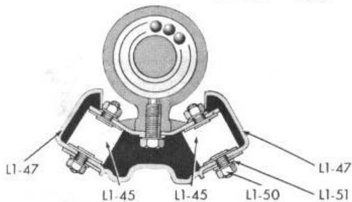
PROPELLER SHAFT WITH SLIDING SPLINE ON REAR SHAFT
